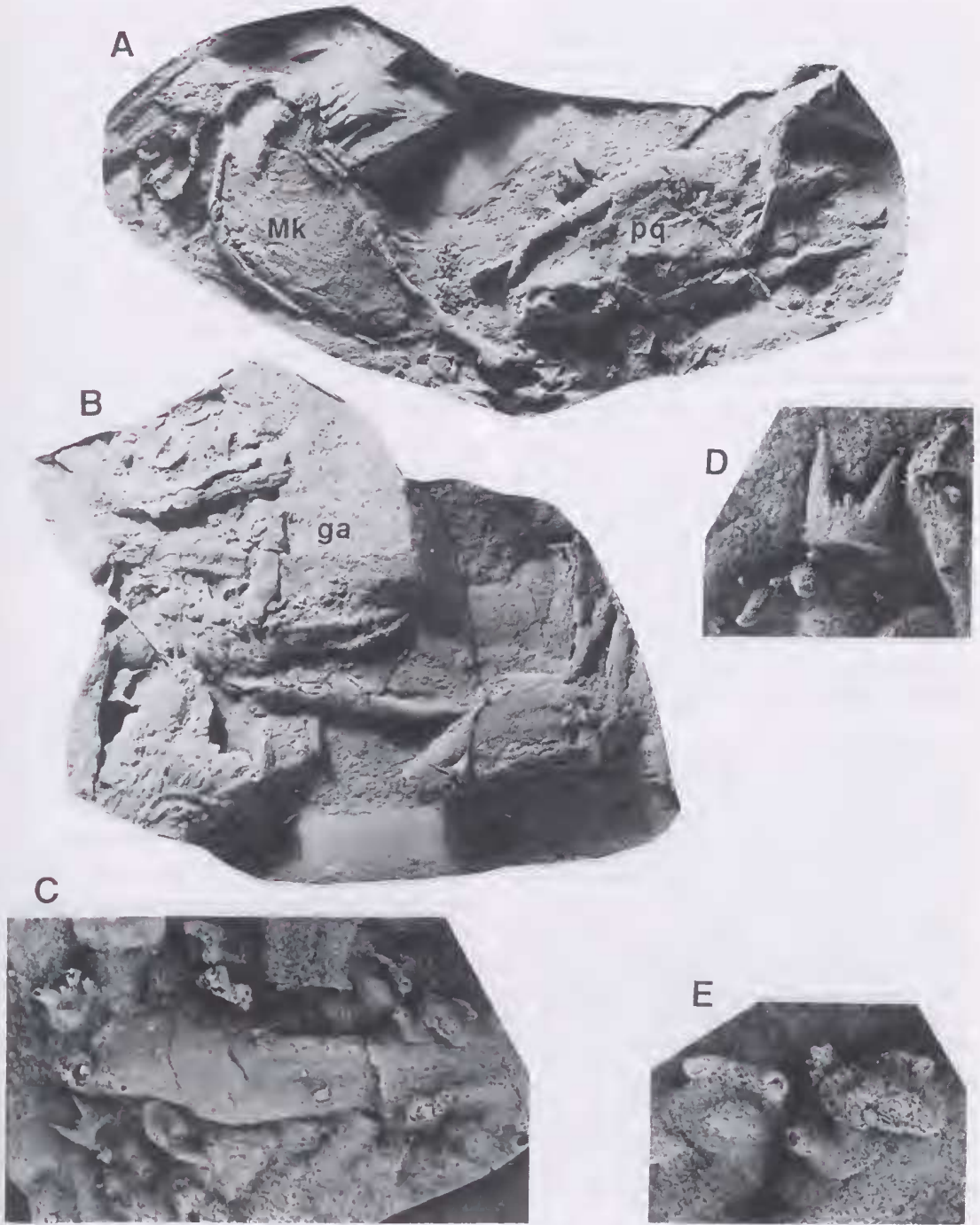
Figure 13 Antarctilamna prisca Young 1982. CPC 21213, Bunga Beds, south coast of New South Wales. A, latex cast showing impressions of the palatoquadrate (pq) previously illustrated by Young (1982, fig. 8C) and associated meckelian cartilage (Mk, x1). B, latex cast of counterpart to A, showing associated gill-arch elements (ga) and teeth (x1). C, detail of gill arch element shown in B, with associated teeth (x 4). D, teeth from lower left of C showing striations on labial side of cusps (upper tooth) and small cusplets lateral to major cusps (lower tooth, base obscure; x 4). E, teeth from top right corner of C showing the button on the lingual torus (x4).
